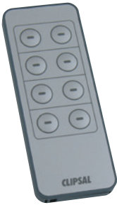
5038TX2 C-Bus 30M 8-Button, Handheld Infrared Remote Control, for C-Bus 30M Switches (also suits Neo Wall Switches, C-Bus Multi-Sensor and 503xNIRL Series Wall Switches)
