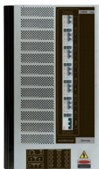
L5112D10UAR6 12-Channel C-Bus Architectural Dimmer, Universal 10A Per Channel (6 RCDs Onboard)
