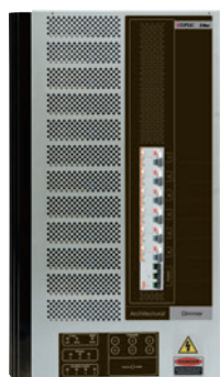
L5106D20UAR6 6-Channel C-Bus Architectural Dimmer, Universal - 20A Per Channel (6 RCDs Onboard)
