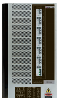
L5112D5UAR6 12-Channel C-Bus Architectural Dimmer, Universal - 5A Per Channel (6 RCDs Onboard)
