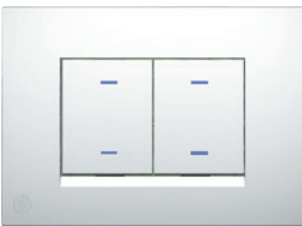
LHC4R4F2 C-Bus Wireless Wall Switch, 4-Button, 2-Channel Relay, 4A (Fluorescent) per Channel Rating Pictured: White
