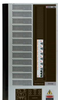
L5106D16UAR6 6-Channel C-Bus Architectural Dimmer, Universal - 16A Per Channel (6 RCDs onboard)
