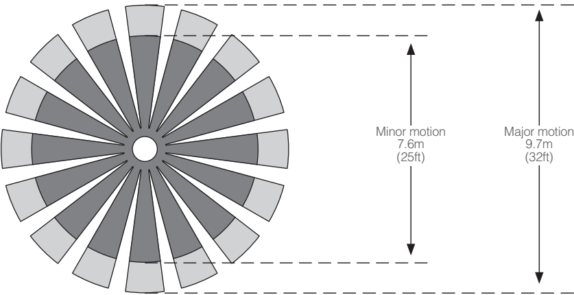
PIR Area of Detection (Top View)
