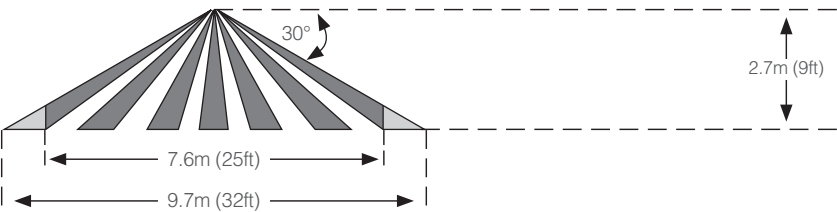
PIR Area of Detection (Side View)
